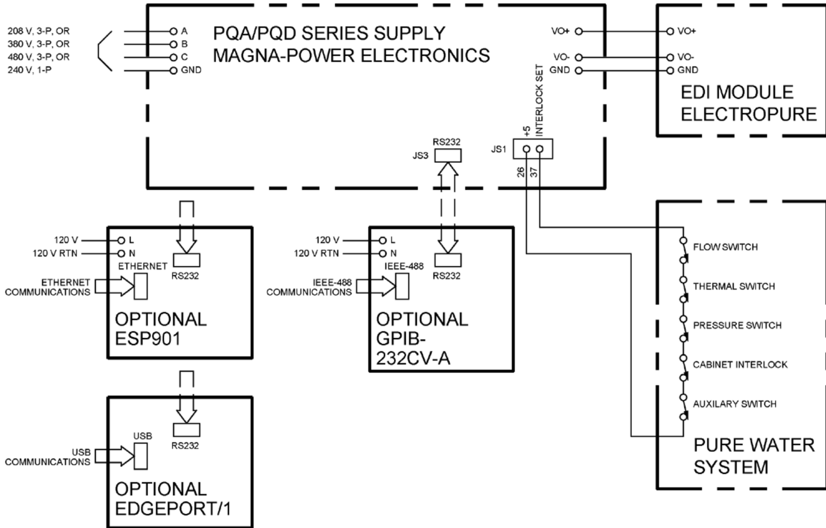
Magna Power EDI Schematic with RS232 – PQA, PQD, SQA, SQA, MQA, MQD, MTA, and MTD Series
