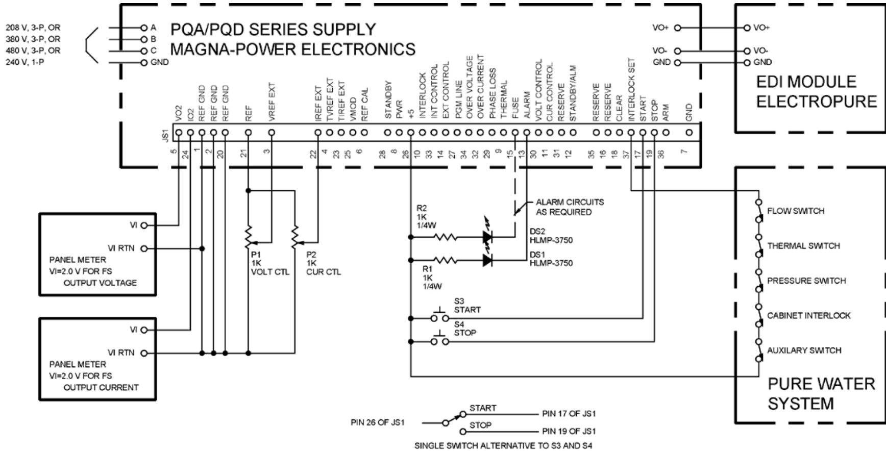
Magna Power Simple EDI Schematic – PQA, PQD, SQA, SQA, MQA, MQD, MTA, and MTD Series
